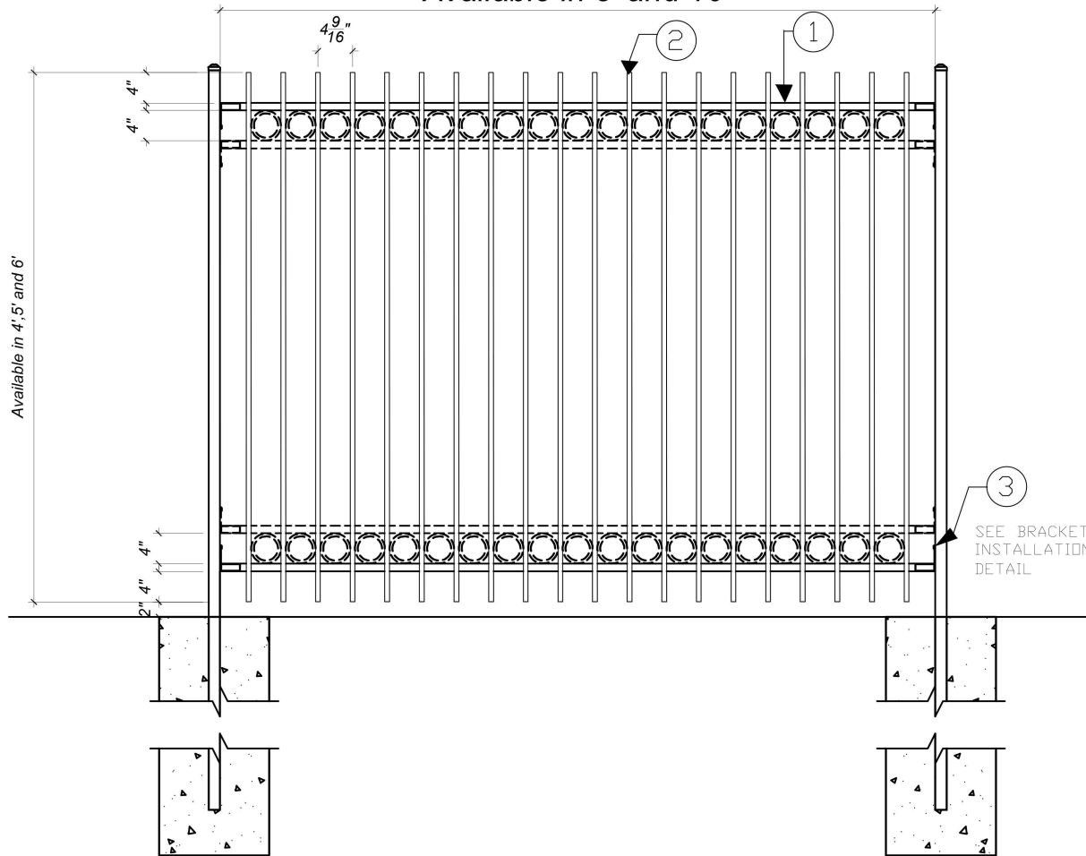
SECTION VIEW
